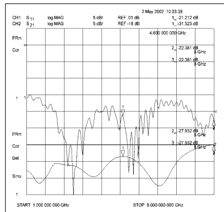
Figure 12 · Reverse coupling and output port return loss.
