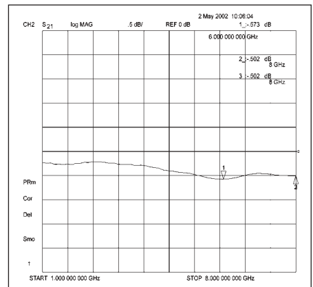
Figure 13 · Insertion loss (vertical scale is 0.5 dB per division).
