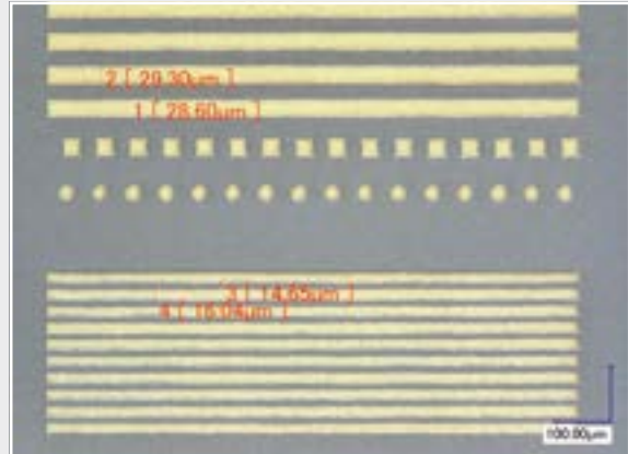
Processing ceramics: Ablation of metal coating, deep engraving, drilling, cutting ( \text{Al}_2\text{O}_3 , GaN)
