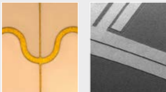
RF structure, Au on Al 2 O 3 ceramic
